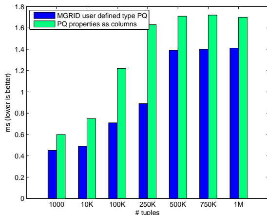
Figure 8: Index equality scan
