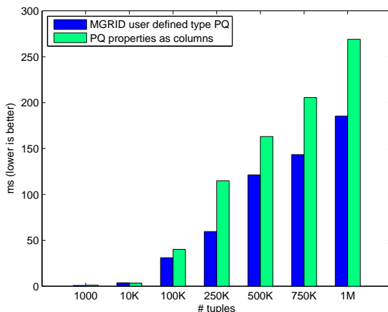
Figure 9: Index range scan
